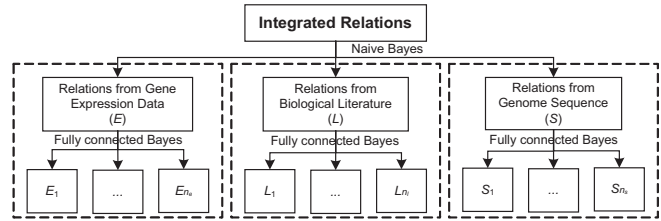
Fig. 2. A two-layered BN for relation integration. Relations from same data sources are integrated using a fully connected BN; and relations from different data sources are integrated using a naive Bayes method.
